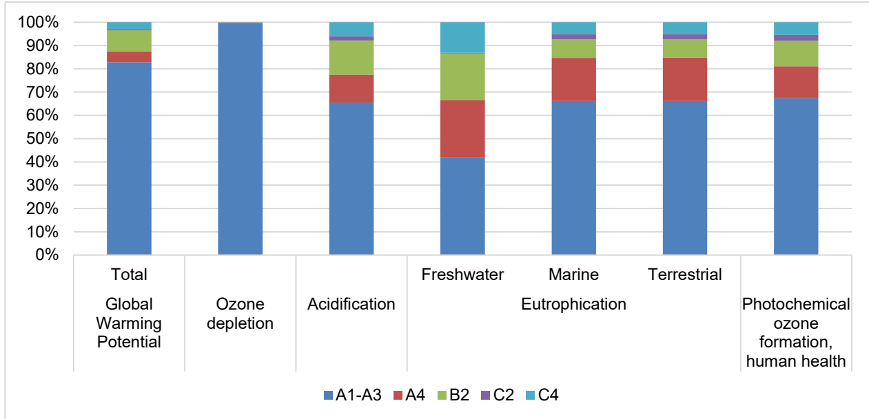
Figure 3 - Relative Contributions of Cradle to Gate Life Cycle Stages for UltraClear™ Flat Glass
