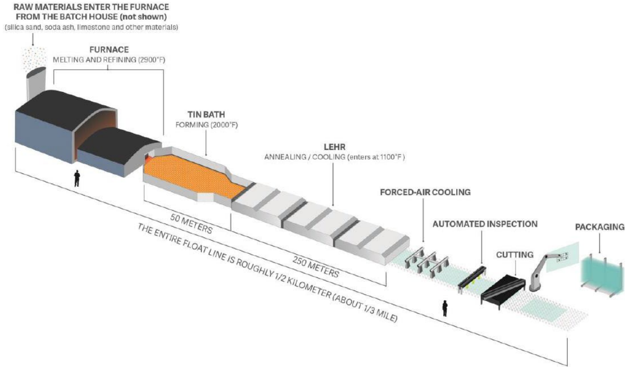
Figure 2 - Flat Glass Production
